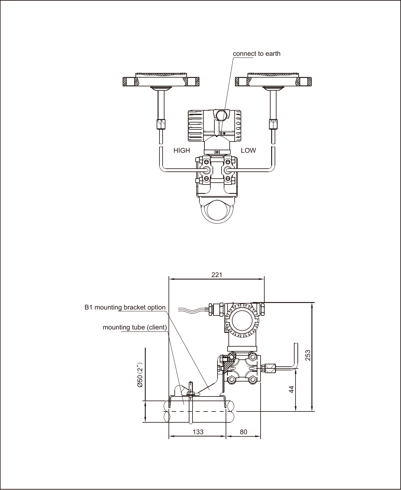
Figure 1 Double-flange remote transmitter installation outline diagram (mm)
