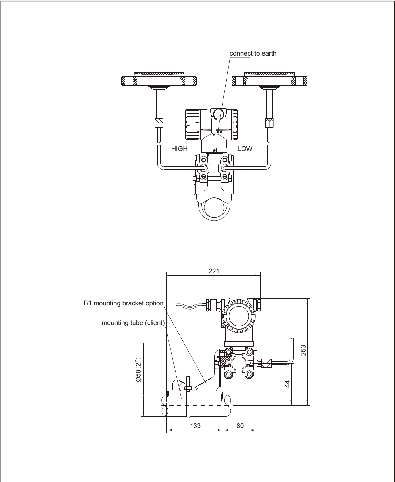
Figure 1 Double-flange remote transmitter installation outline diagram (mm)
